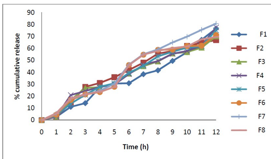
Figure: Graph showing % cumulative drug release vs time of the prepared formulations
